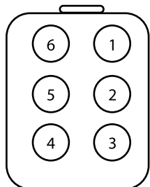
Figure 2: Connector 2 Pinout
