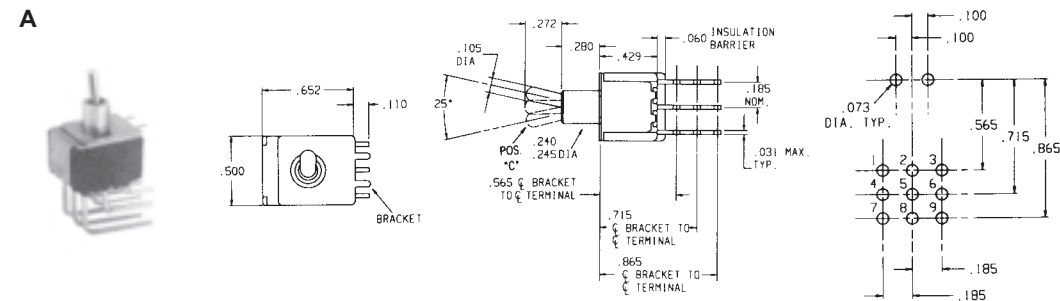
Three Pole
