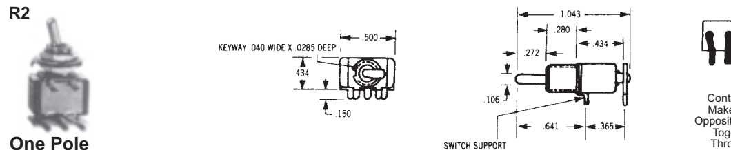
One Pole
